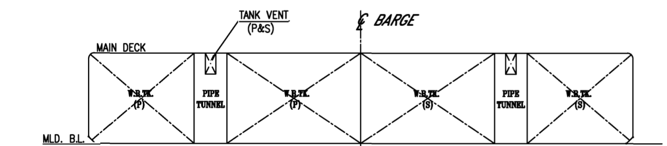
SECTION AT TANKS
