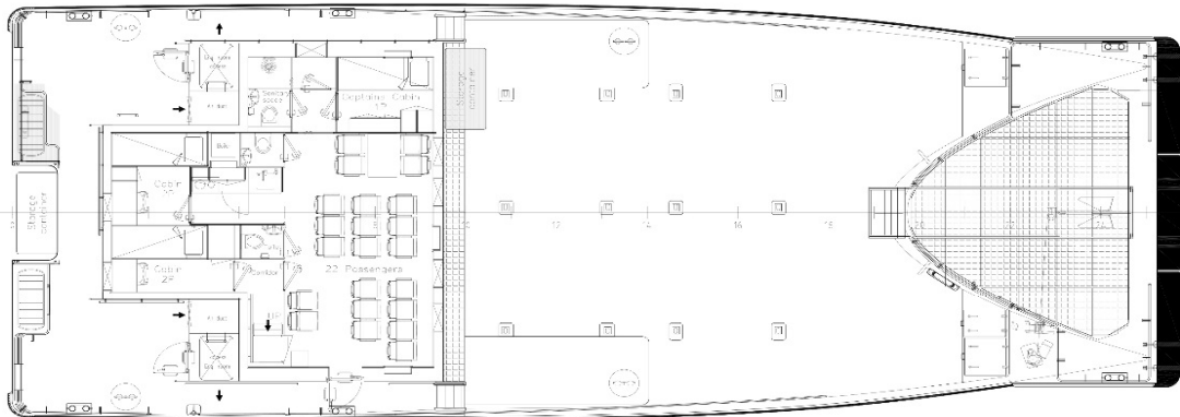
Main deck
