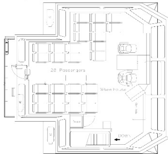
Bridge deck
